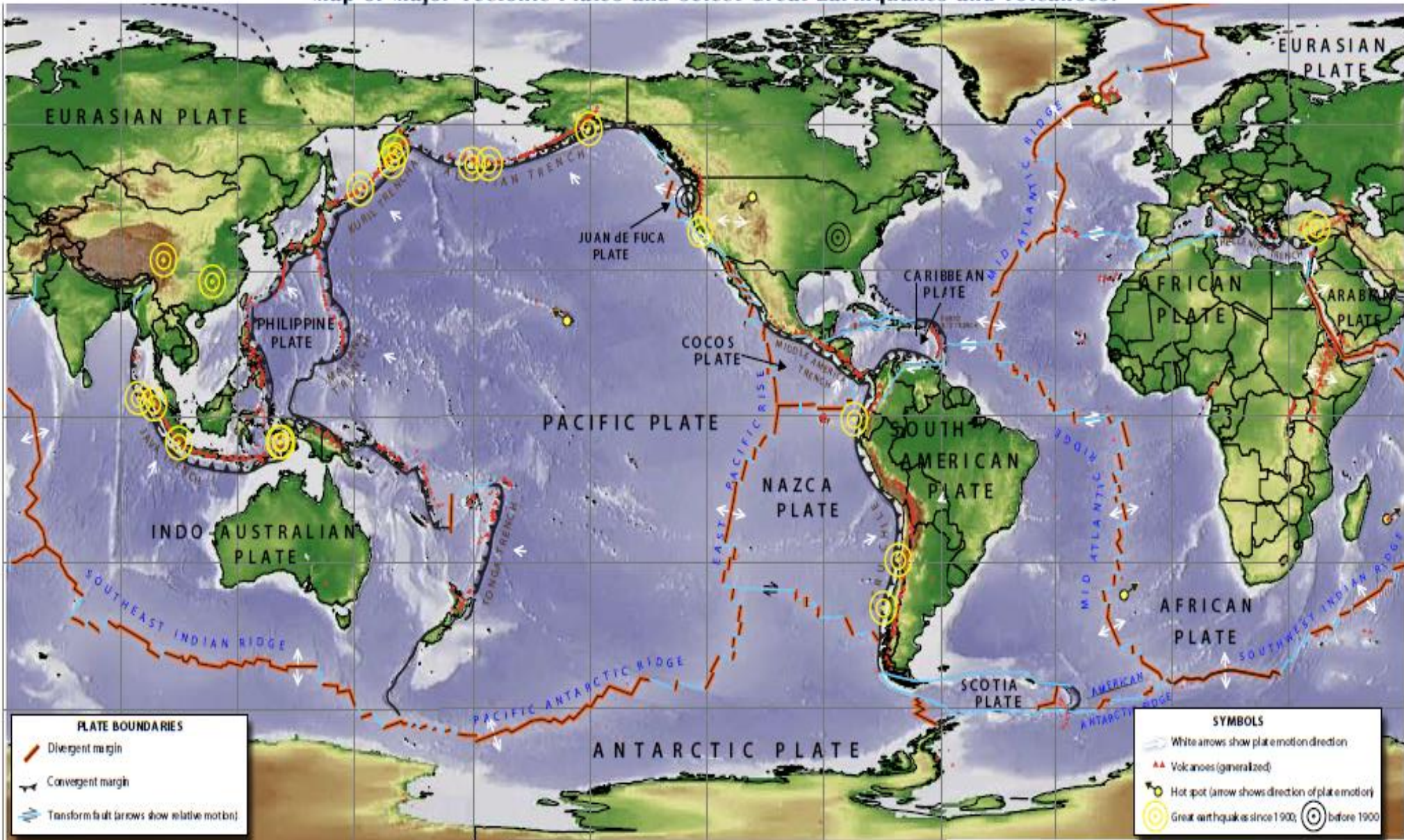
map of major tectonic plates and select Great Earthquakes and volcanoes.
